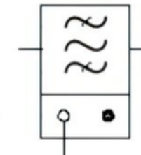
Band-pass filter switched by gas discharge
